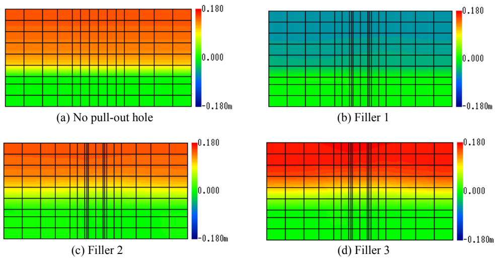
Fig. 5 X-direction displacement contour diagrams
