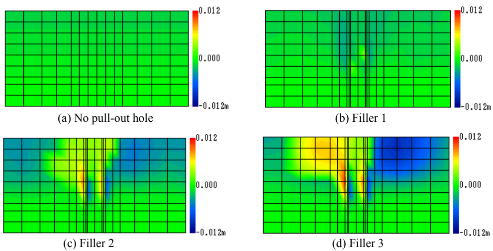
Fig. 6 Y-direction displacement contour diagrams
