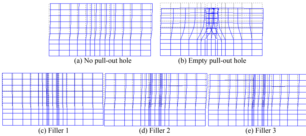
Fig. 4 Displacement diagram (The amount of displacement is three times)
