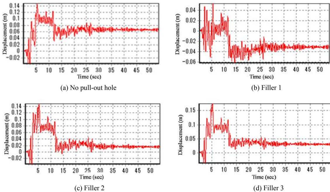
Fig. 7 Time history view of the X-direction displacement of the ground centre
