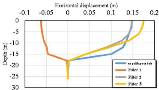
Fig. 8 Graph comparing the horizontal displacements of the ground centre line
