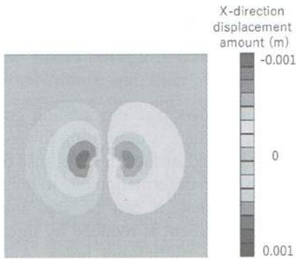
(b) Filler 1 ( q_u=0.1 )
