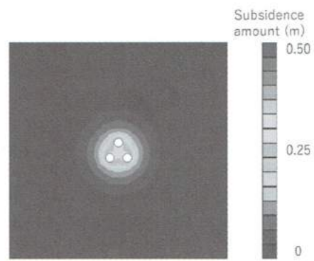
(a) Pulling-out holes are hollow
