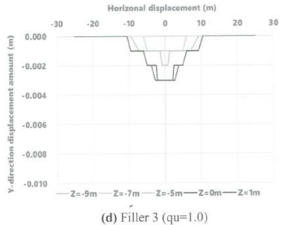
Figure5 Settlement amount graph at ground surface
