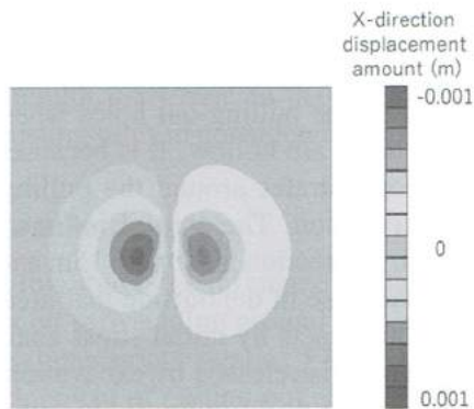
(c) Filler 2 ( q_u=0.5 )
