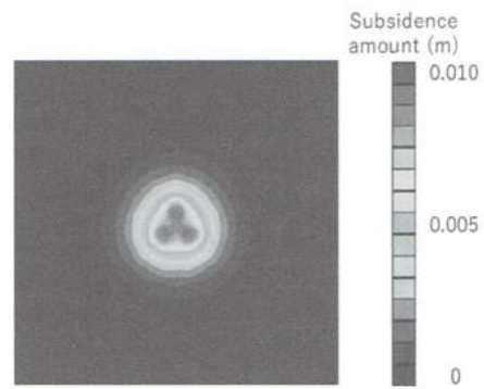
(b) Filler 1 ( q_u=0.1 )
