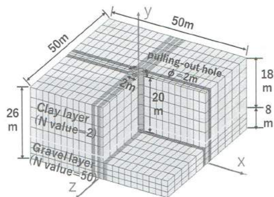
(a) When the pulling-out holes are hollow
