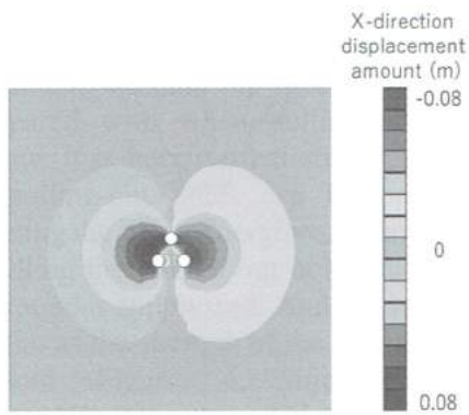
(a) Pulling-out holes are hollow
