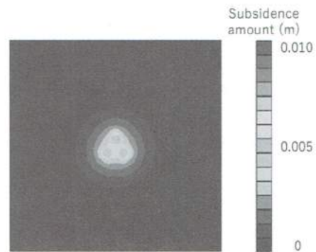
(c) Filler 2 ( q_u=0.5 )
